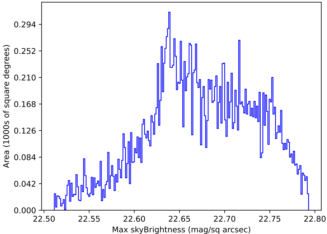
too_elab_r128_d3_ugrizy_v3.4_10yrs Yr 1 u band: Max skyBrightness
