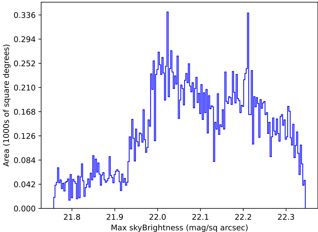
too_elab_r128_d3_ugrizy_v3.4_10yrs Yr 1 g band: Max skyBrightness
