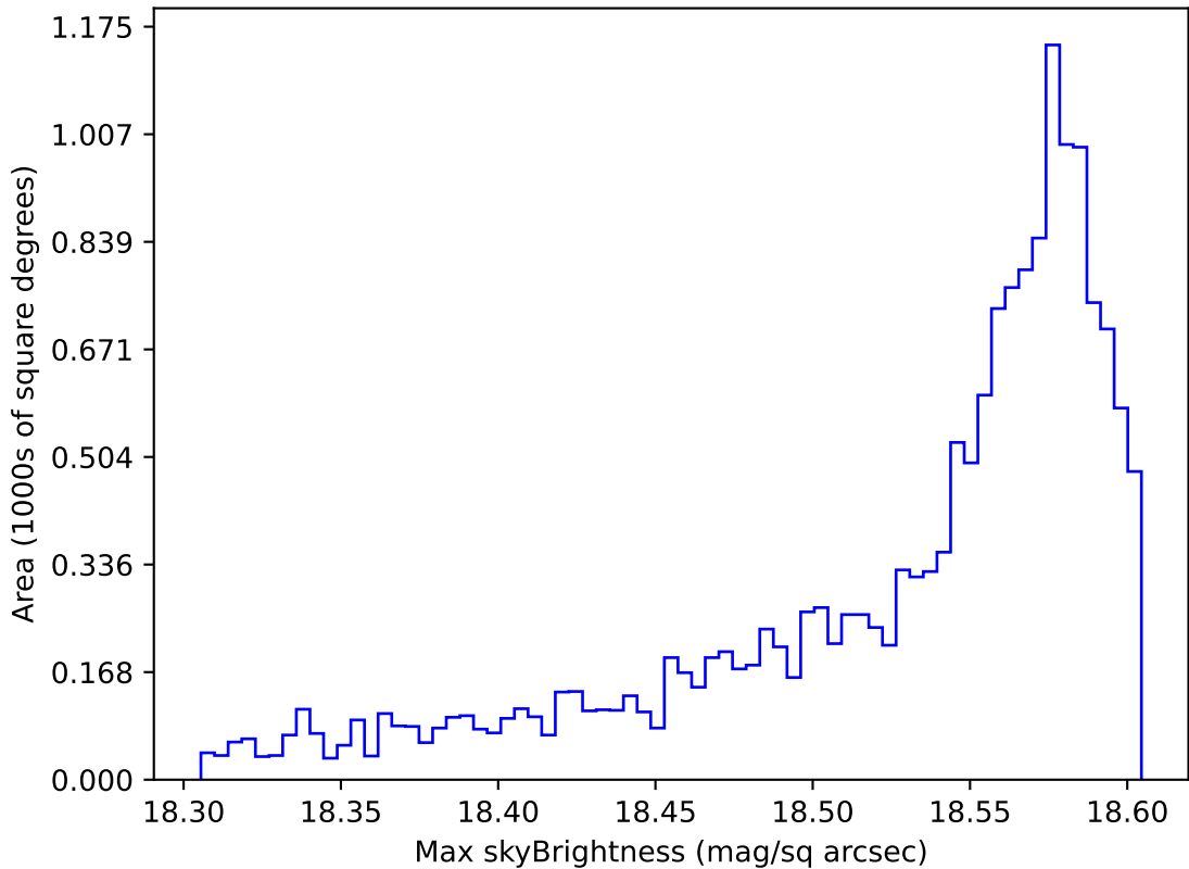
too_elab_r128_d3_ugrizy_v3.4_10yrs WFD y band: Max skyBrightness
