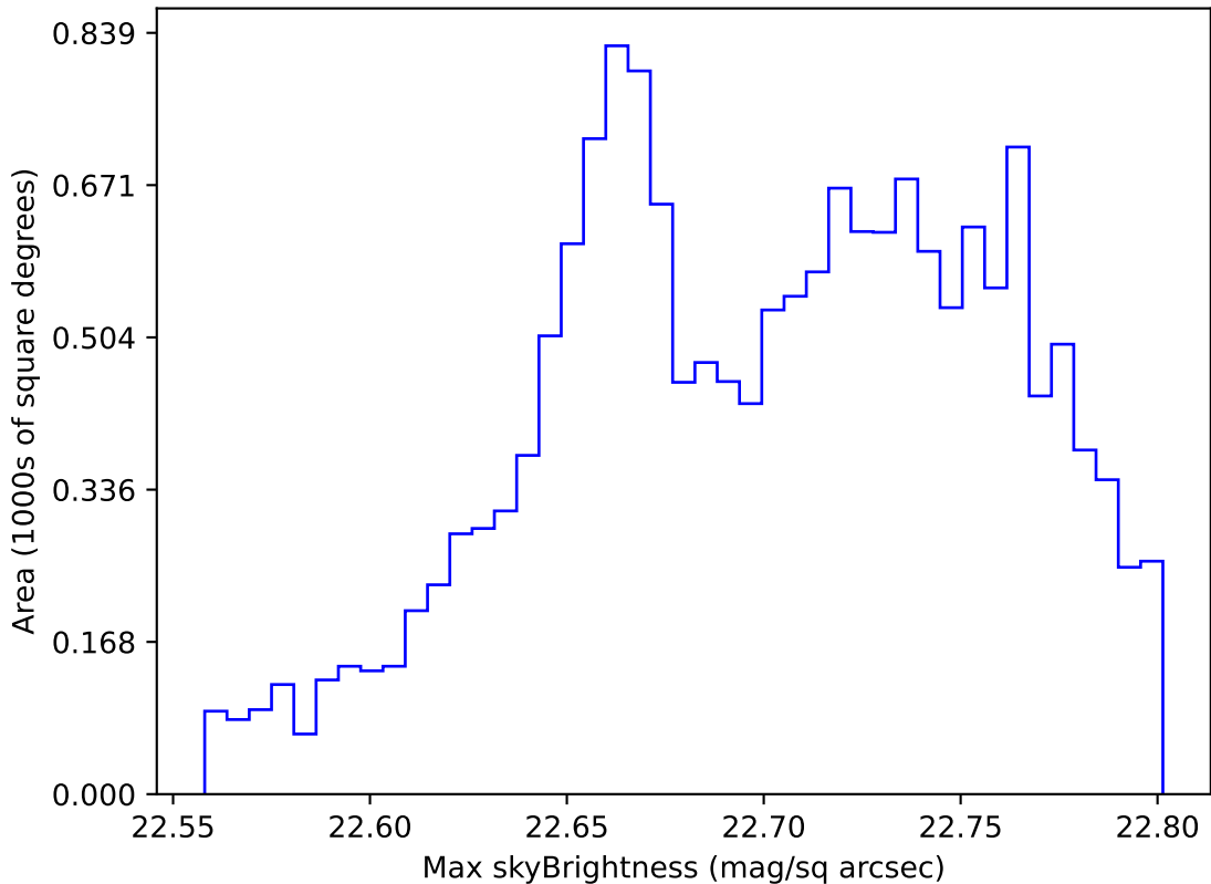
too_elab_r128_d3_ugrizy_v3.4_10yrs WFD u band: Max skyBrightness
