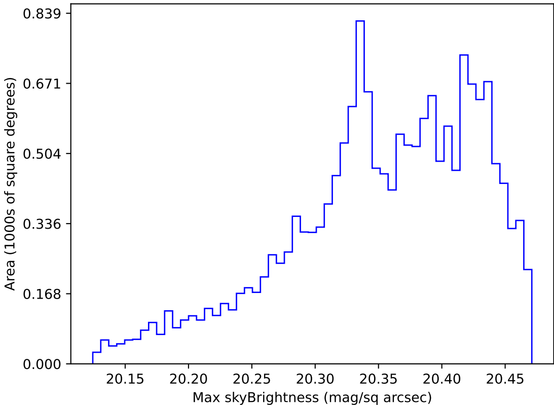
too_elab_r128_d3_ugrizy_v3.4_10yrs WFD i band: Max skyBrightness
