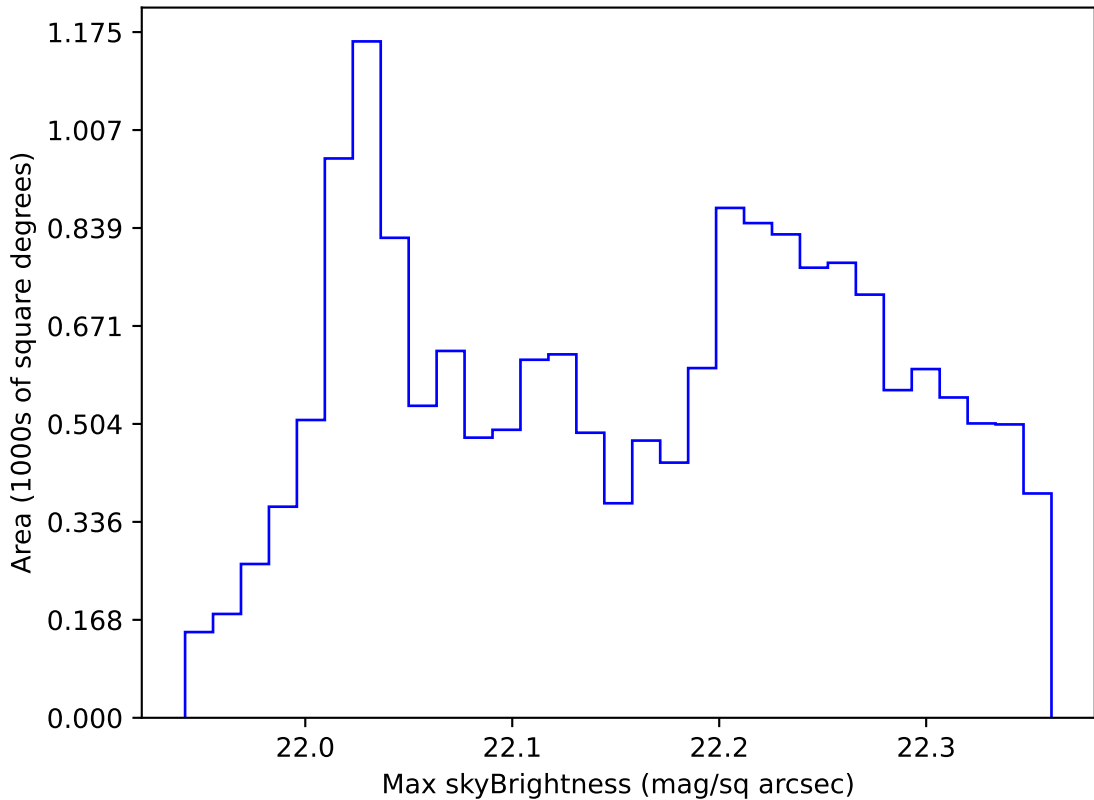
too_elab_r128_d3_ugrizy_v3.4_10yrs WFD g band: Max skyBrightness
