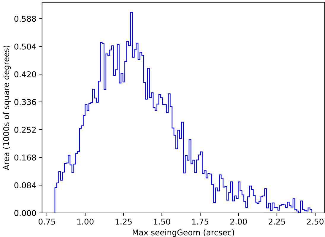
too_elab_r128_d3_ugrizy_v3.4_10yrs Yr 1 g band: Max seeingGeom
