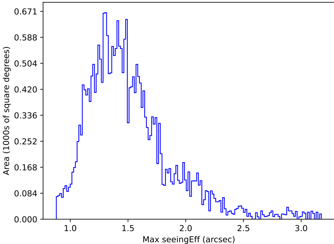
too_elab_r128_d3_ugrizy_v3.4_10yrs Yr 1 z band: Max seeingEff
