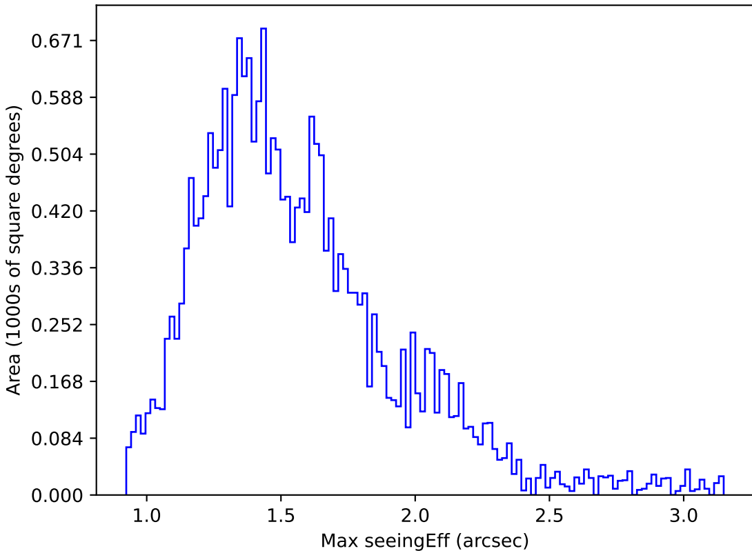
too_elab_r128_d3_ugrizy_v3.4_10yrs Yr 1 u band: Max seeingEff
