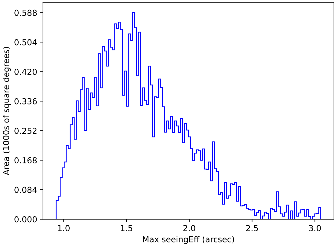
too_elab_r128_d3_ugrizy_v3.4_10yrs Yr 1 r band: Max seeingEff
