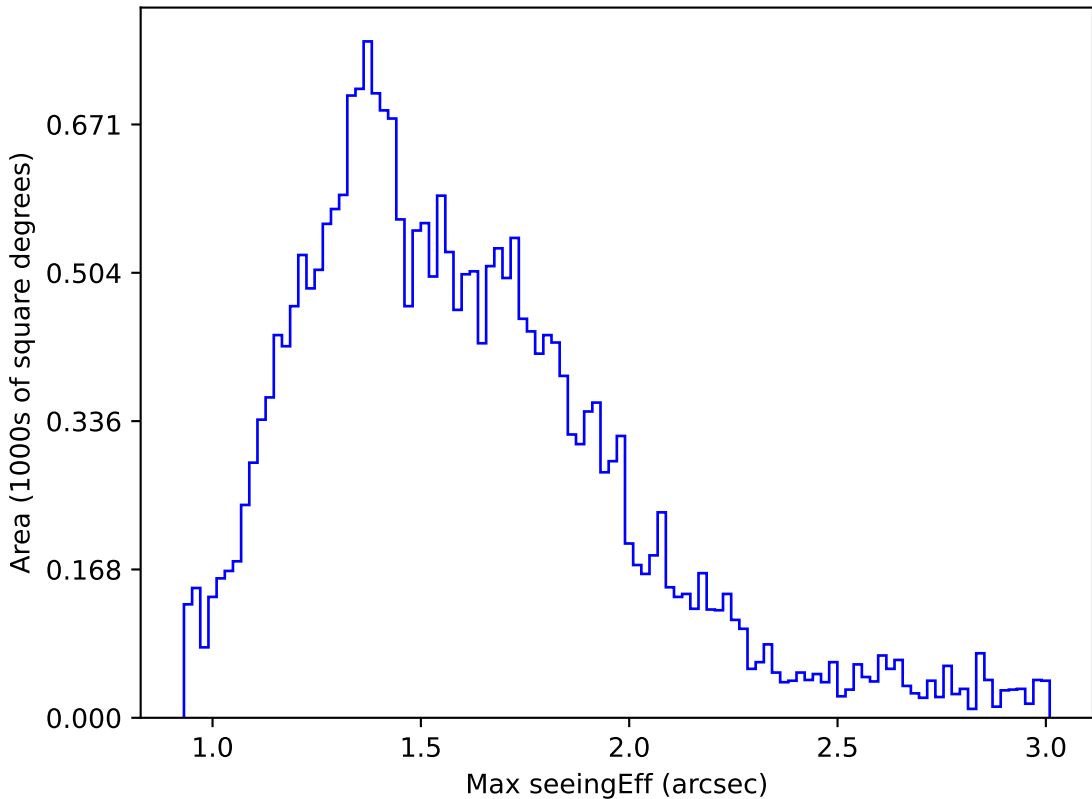
too_elab_r128_d3_ugrizy_v3.4_10yrs Yr 1 i band: Max seeingEff
