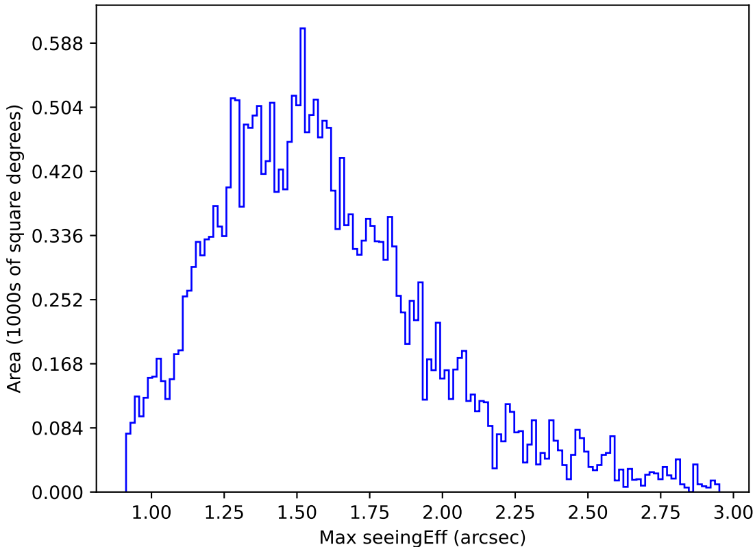
too_elab_r128_d3_ugrizy_v3.4_10yrs Yr 1 g band: Max seeingEff
