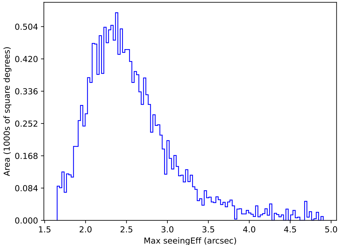
too_elab_r128_d3_ugrizy_v3.4_10yrs WFD z band: Max seeingEff
