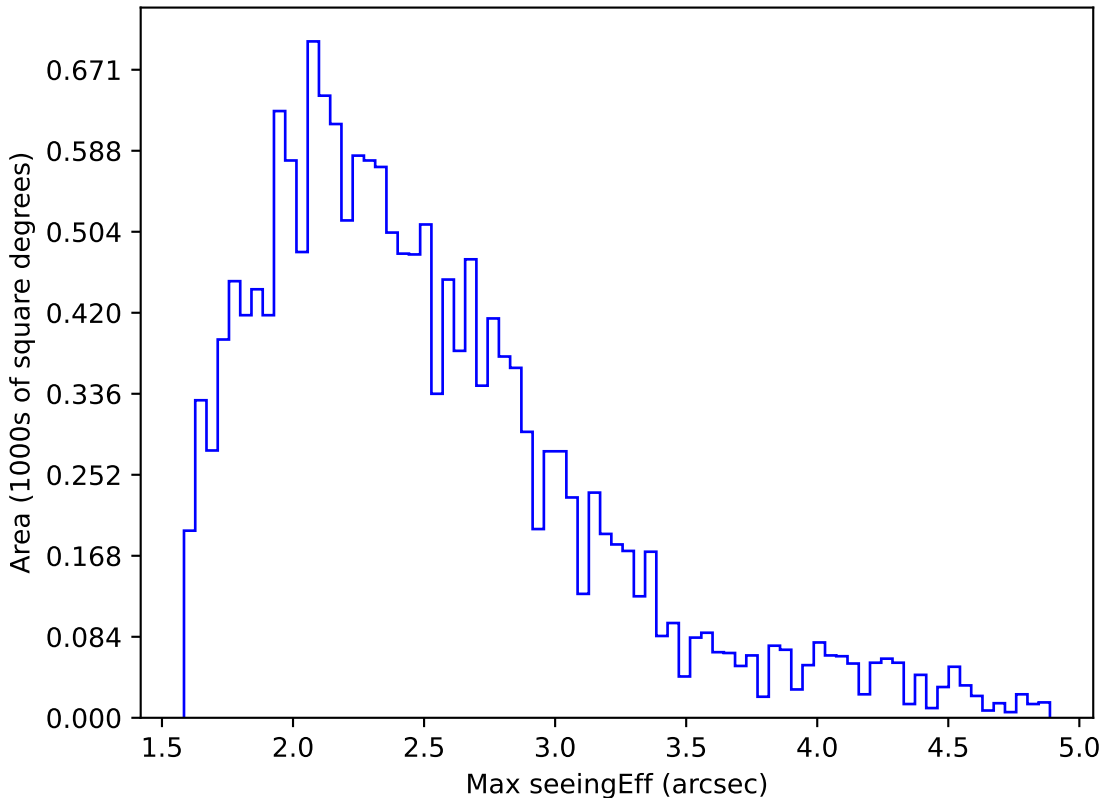
too_elab_r128_d3_ugrizy_v3.4_10yrs WFD y band: Max seeingEff
