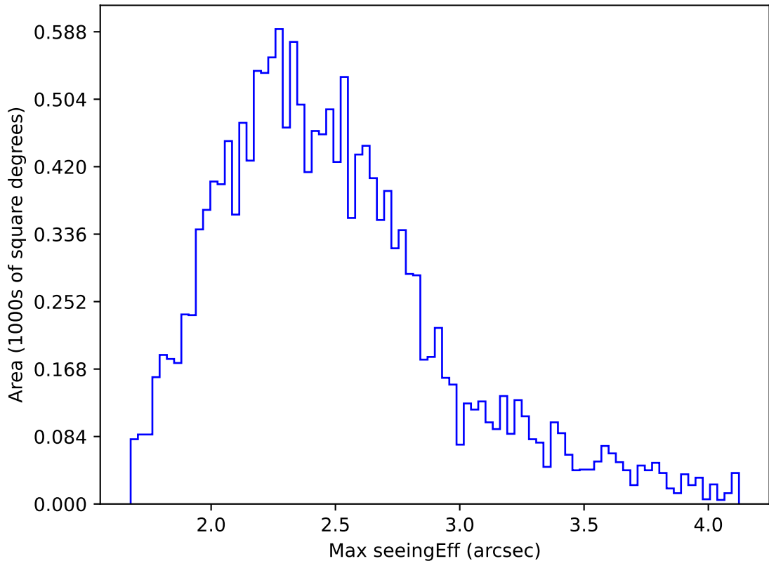
too_elab_r128_d3_ugrizy_v3.4_10yrs WFD u band: Max seeingEff
