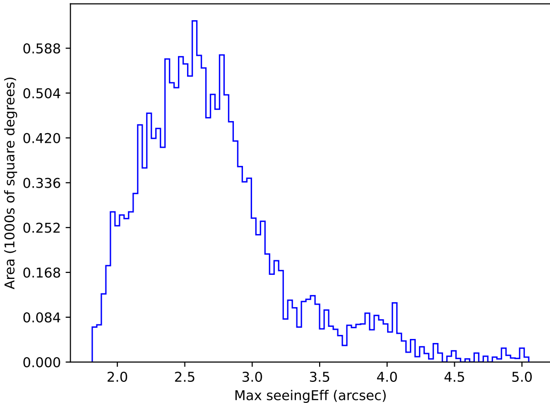
too_elab_r128_d3_ugrizy_v3.4_10yrs WFD r band: Max seeingEff
