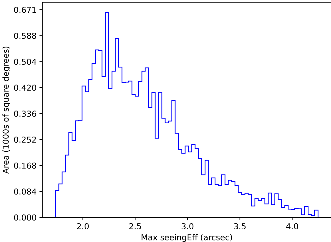
too_elab_r128_d3_ugrizy_v3.4_10yrs WFD g band: Max seeingEff
