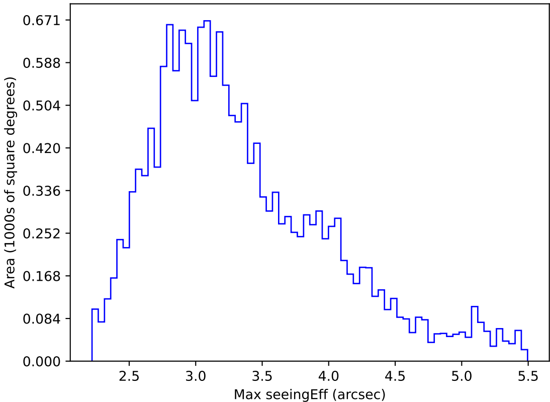
too_elab_r128_d3_ugrizy_v3.4_10yrs WFD all bands: Max seeingEff
