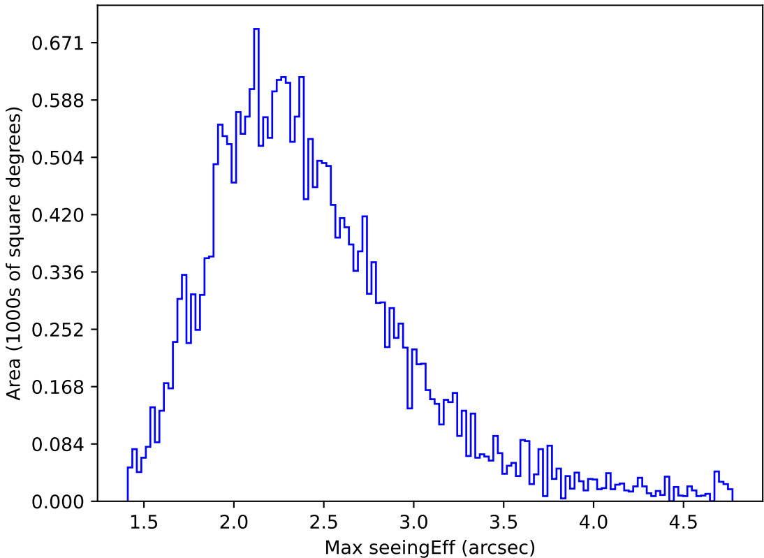
too_elab_r128_d3_ugrizy_v3.4_10yrs All sky z band: Max seeingEff
