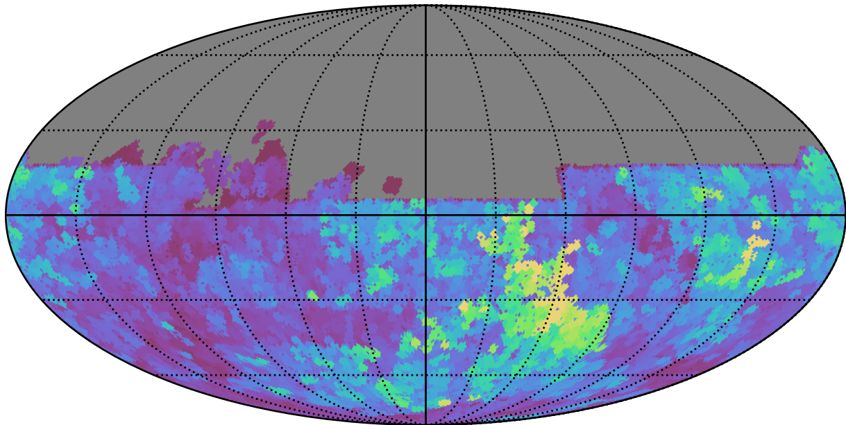
too_elab_r128_d3_ugrizy_v3.4_10yrs All sky y band: Max seeingEff
