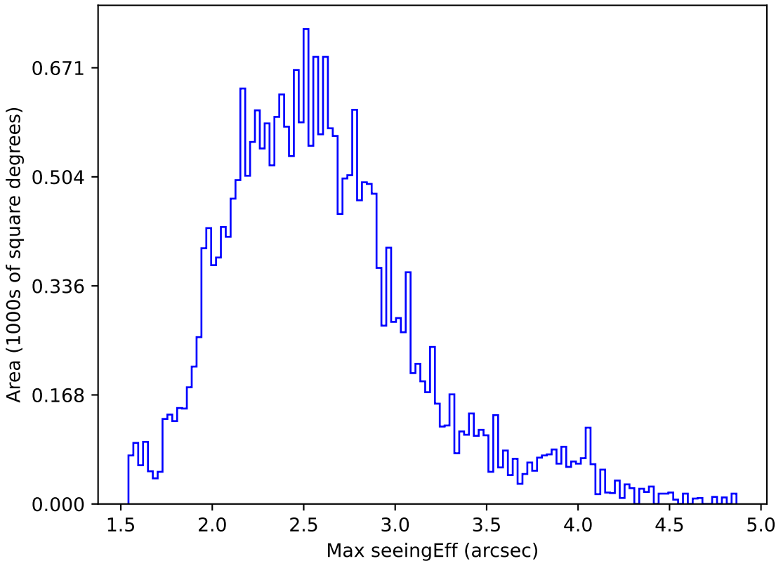
too_elab_r128_d3_ugrizy_v3.4_10yrs All sky r band: Max seeingEff
