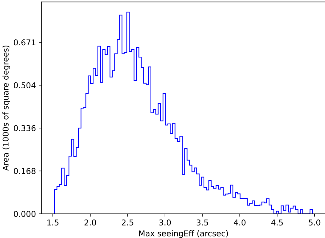
too_elab_r128_d3_ugrizy_v3.4_10yrs All sky i band: Max seeingEff
