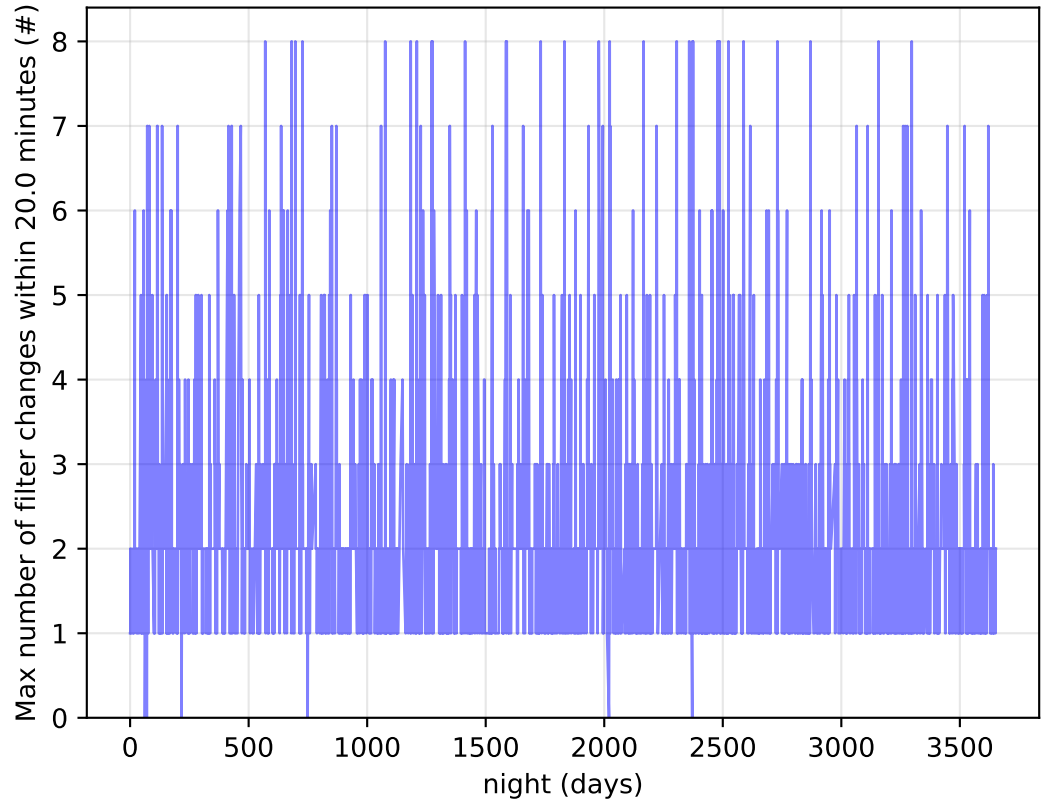
too_elab_r128_d3_ugrizy_v3.4_10yrs Per Night: Max number of filter changes within 20.0 minutes
