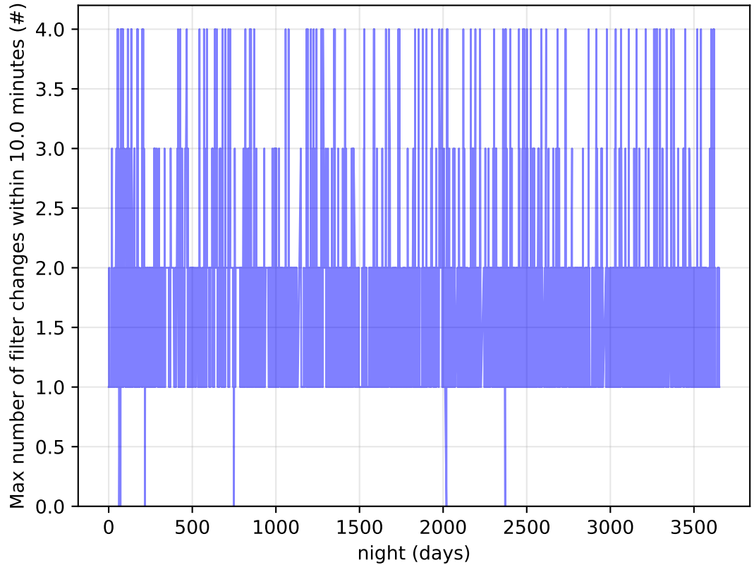
too_elab_r128_d3_ugrizy_v3.4_10yrs Per Night: Max number of filter changes within 10.0 minutes
