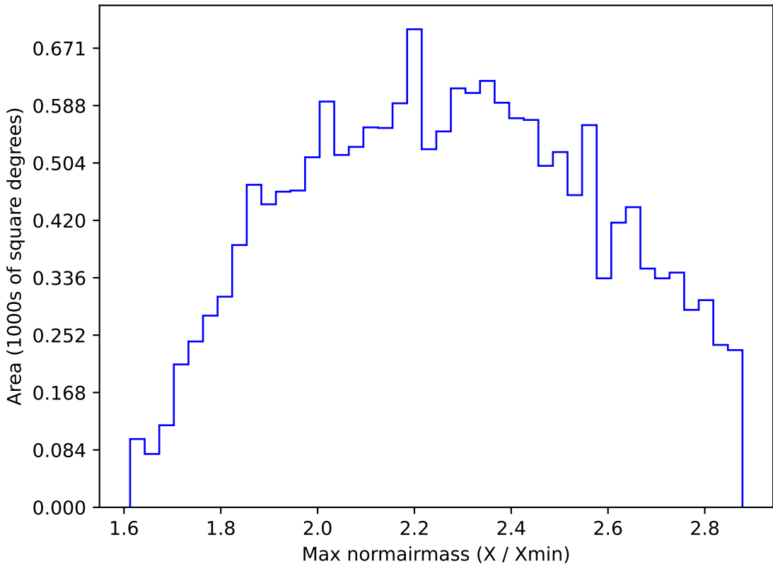
too_elab_r128_d3_ugrizy_v3.4_10yrs WFD z band: Max normairmass
