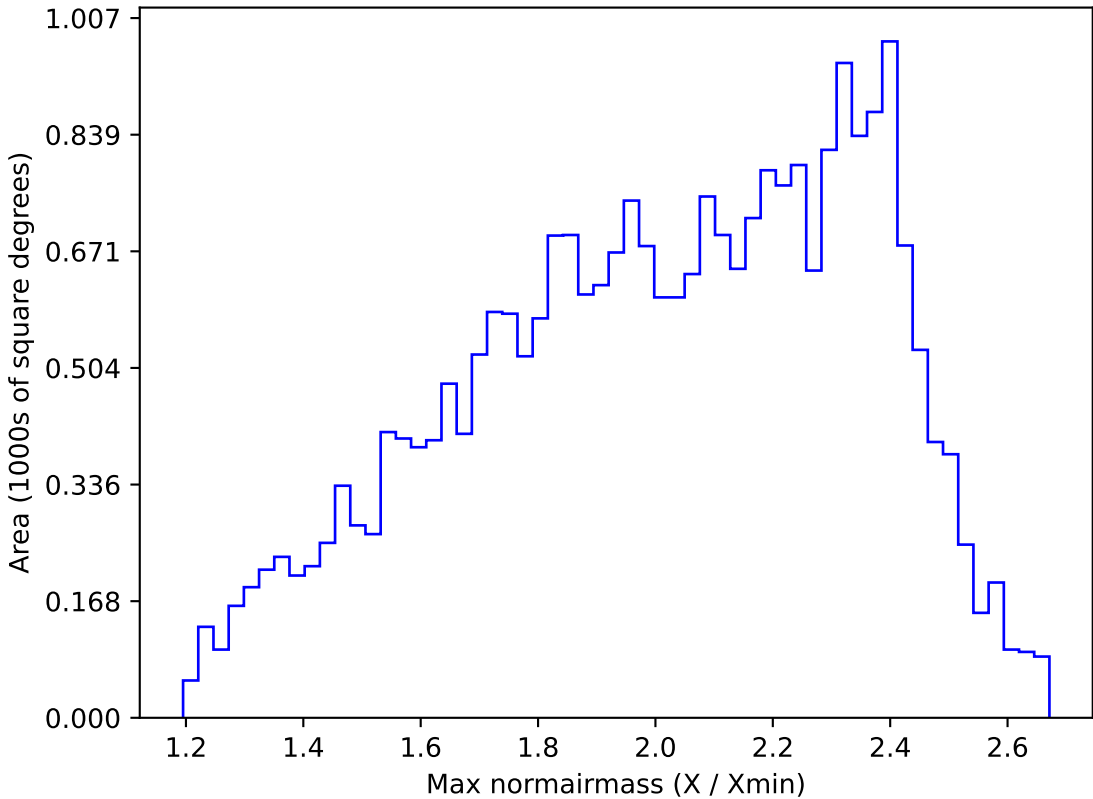
too_elab_r128_d3_ugrizy_v3.4_10yrs All sky r band: Max normairmass
