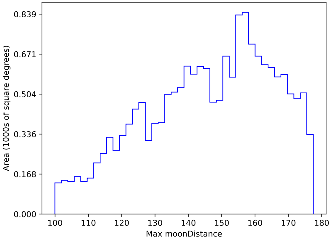
too_elab_r128_d3_ugrizy_v3.4_10yrs WFD y band: Max moonDistance
