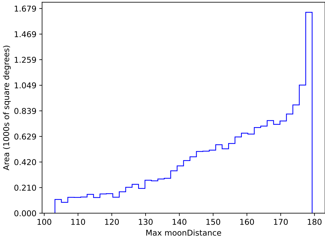
too_elab_r128_d3_ugrizy_v3.4_10yrs WFD r band: Max moonDistance
