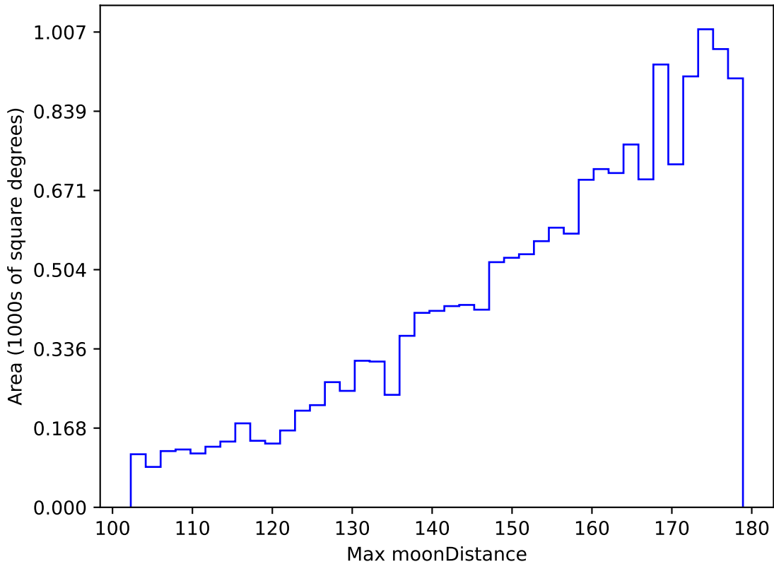
too_elab_r128_d3_ugrizy_v3.4_10yrs WFD g band: Max moonDistance
