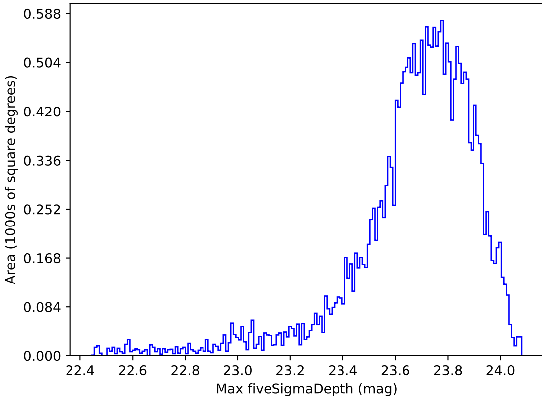
too_elab_r128_d3_ugrizy_v3.4_10yrs All sky u band: Max fiveSigmaDepth
