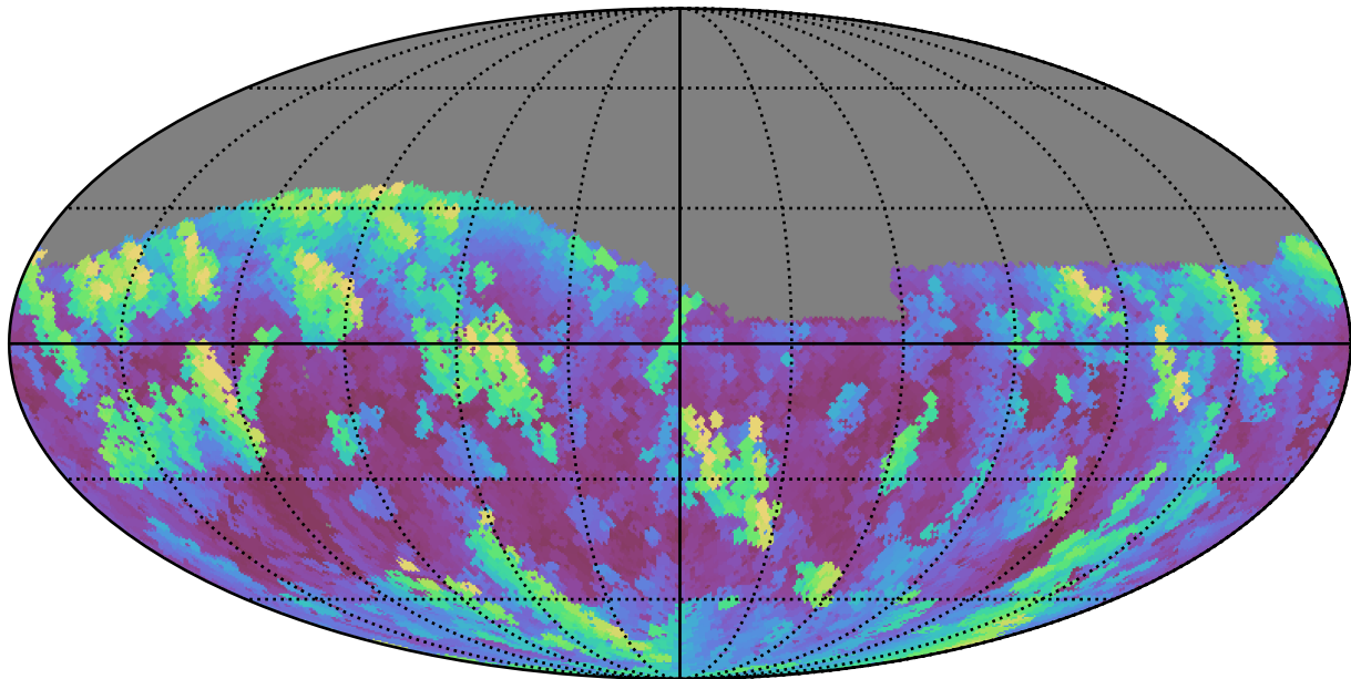
too_elab_r128_d3_ugrizy_v3.4_10yrs Yr 1 z band: Max airmass
