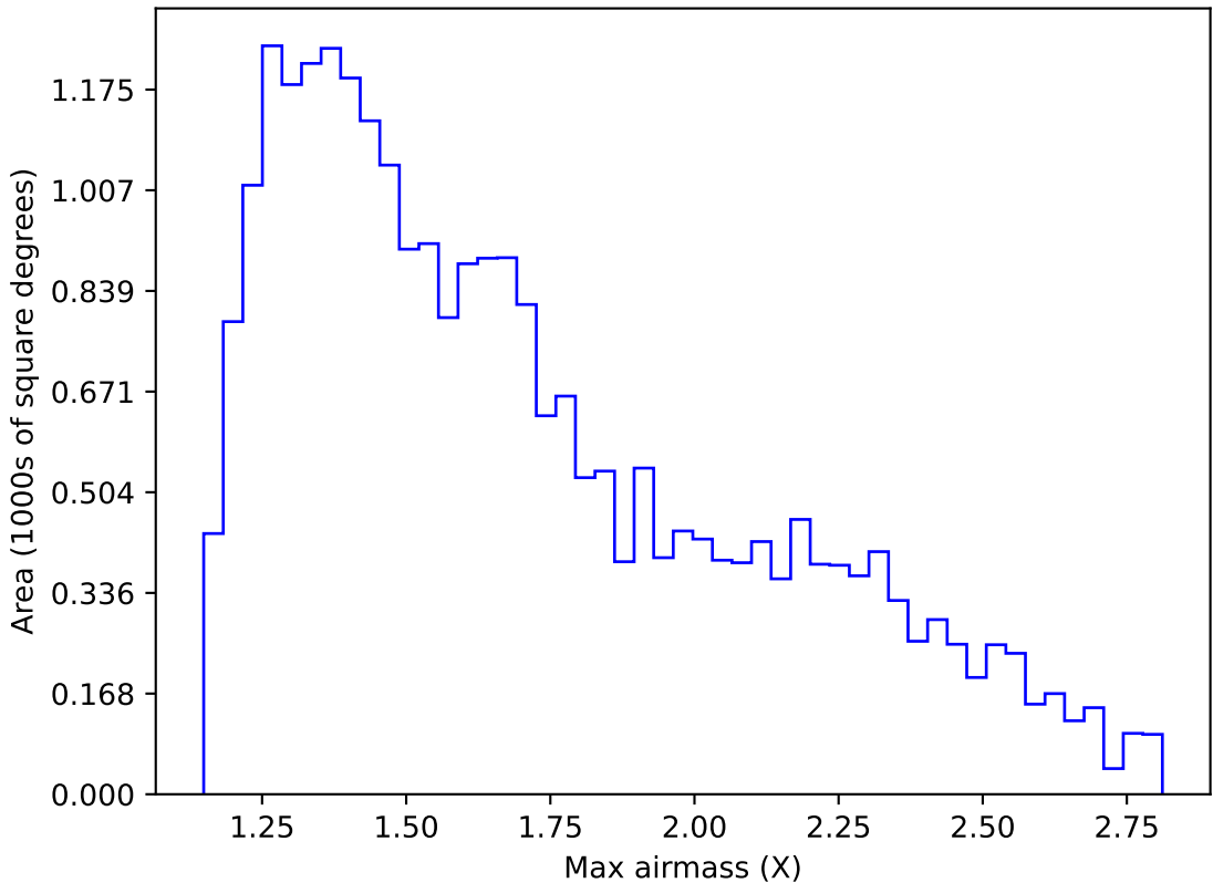
too_elab_r128_d3_ugrizy_v3.4_10yrs Yr 1 z band: Max airmass
