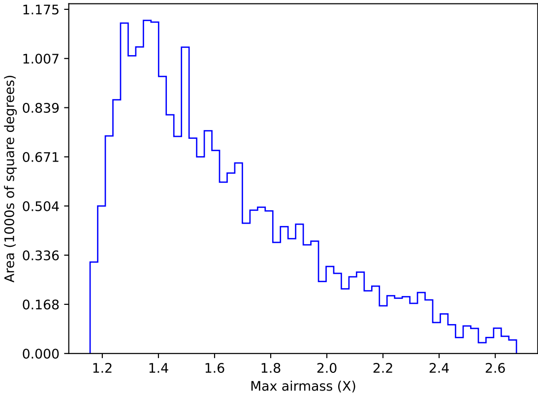
too_elab_r128_d3_ugrizy_v3.4_10yrs Yr 1 y band: Max airmass
