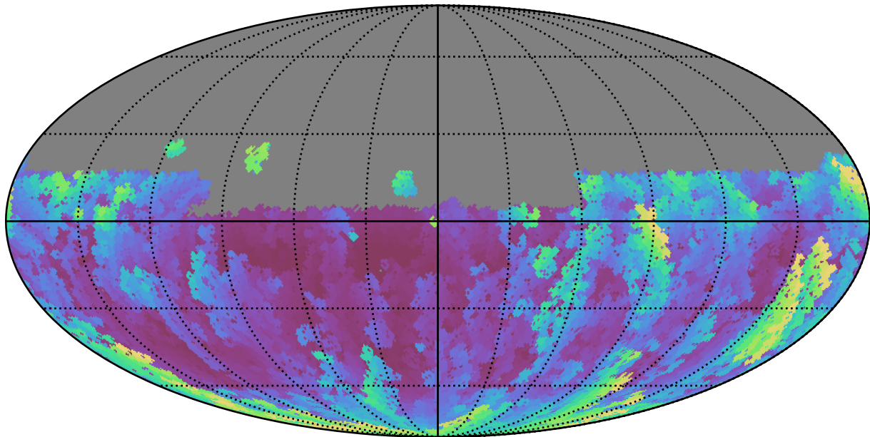
too_elab_r128_d3_ugrizy_v3.4_10yrs Yr 1 u band: Max airmass
