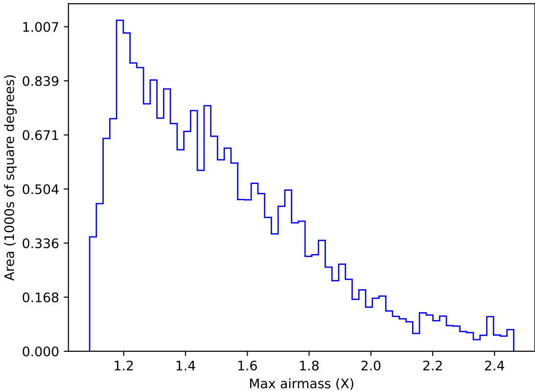
too_elab_r128_d3_ugrizy_v3.4_10yrs Yr 1 u band: Max airmass
