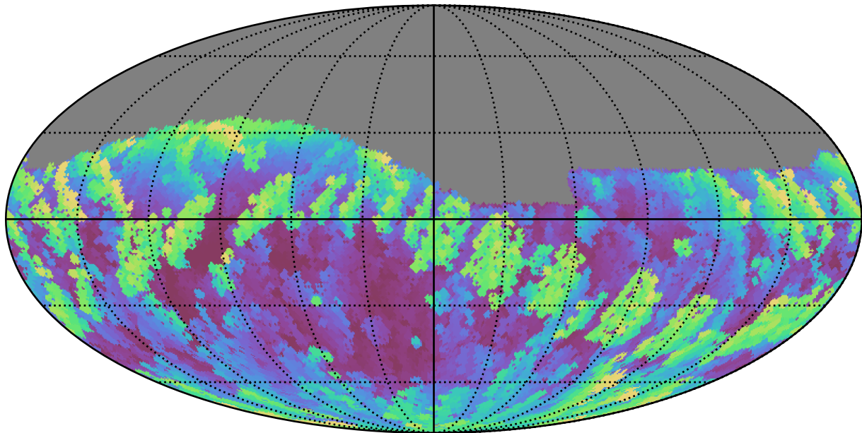
too_elab_r128_d3_ugrizy_v3.4_10yrs Yr 1 r band: Max airmass
