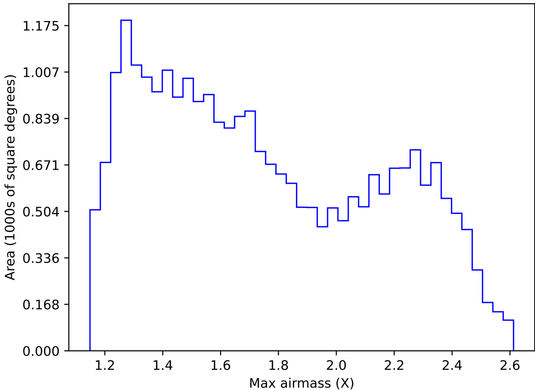
too_elab_r128_d3_ugrizy_v3.4_10yrs Yr 1 r band: Max airmass
