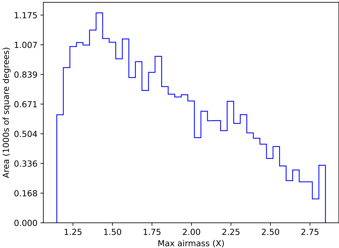
too_elab_r128_d3_ugrizy_v3.4_10yrs Yr 1 i band: Max airmass
