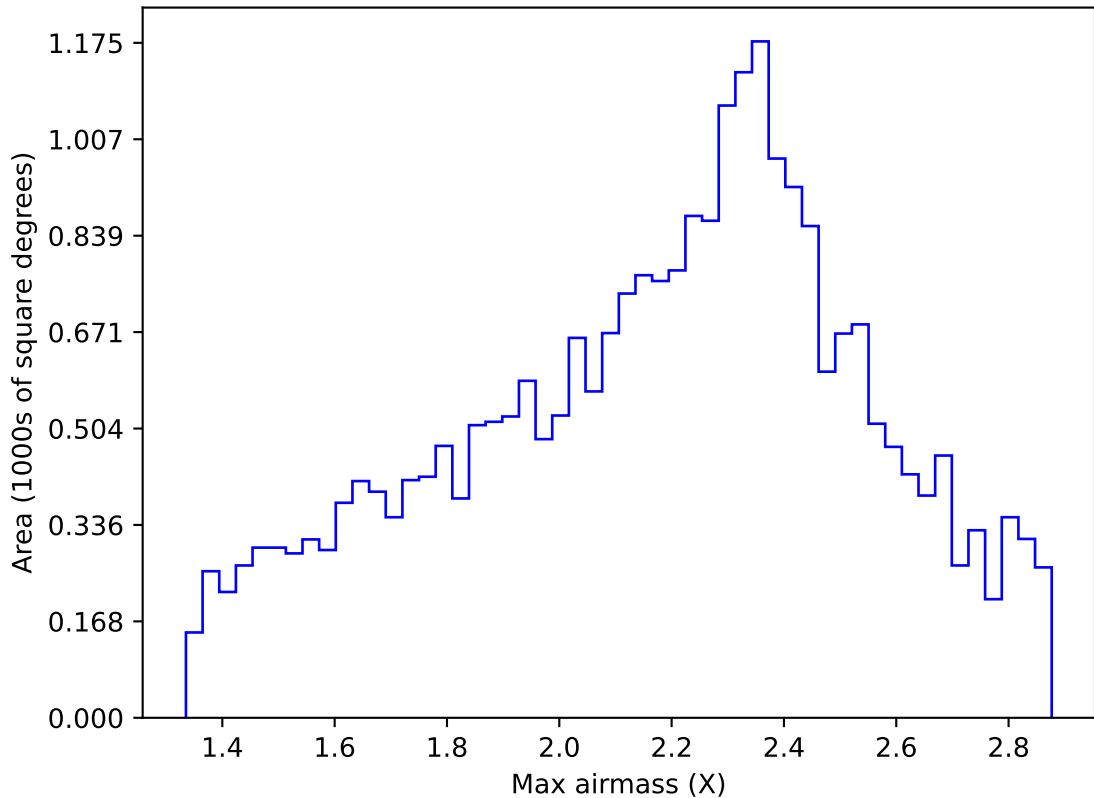
too_elab_r128_d3_ugrizy_v3.4_10yrs Yr 1 all bands: Max airmass
