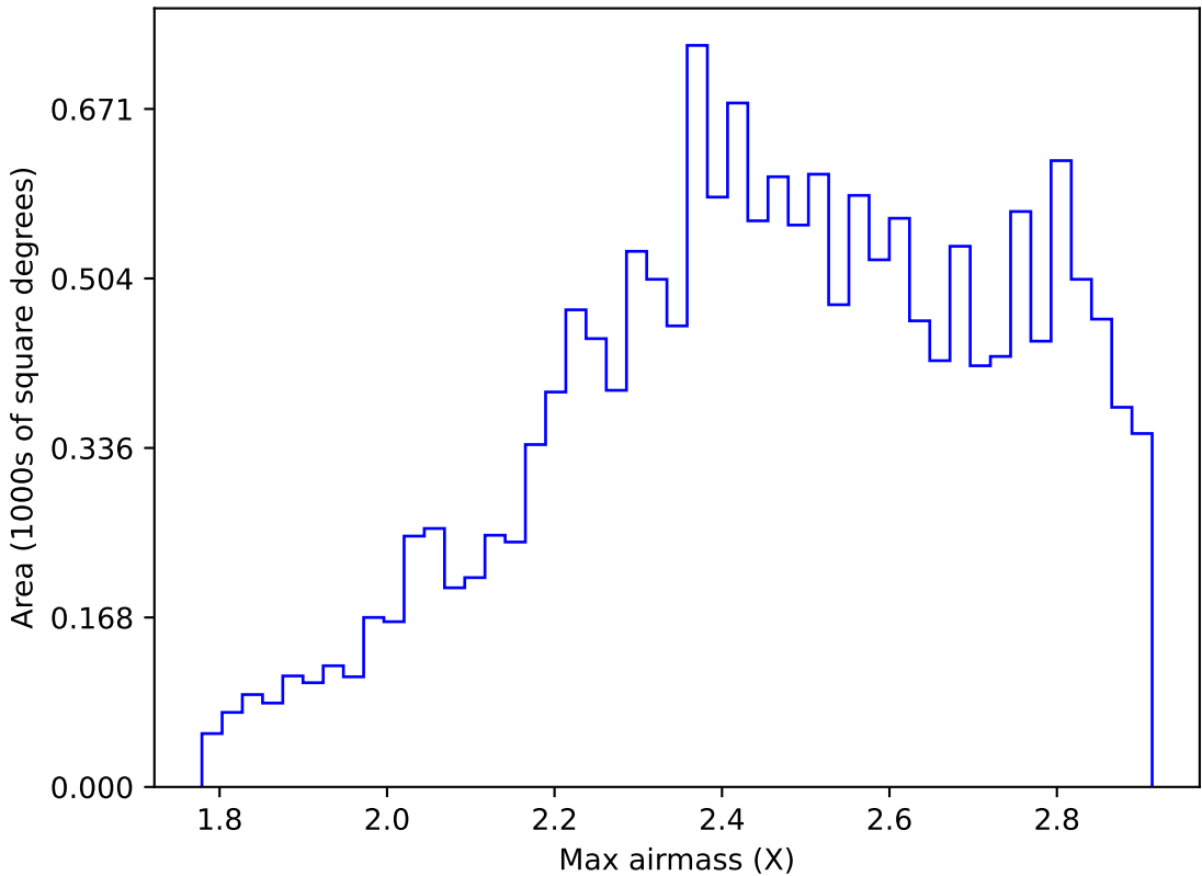
too_elab_r128_d3_ugrizy_v3.4_10yrs WFD z band: Max airmass
