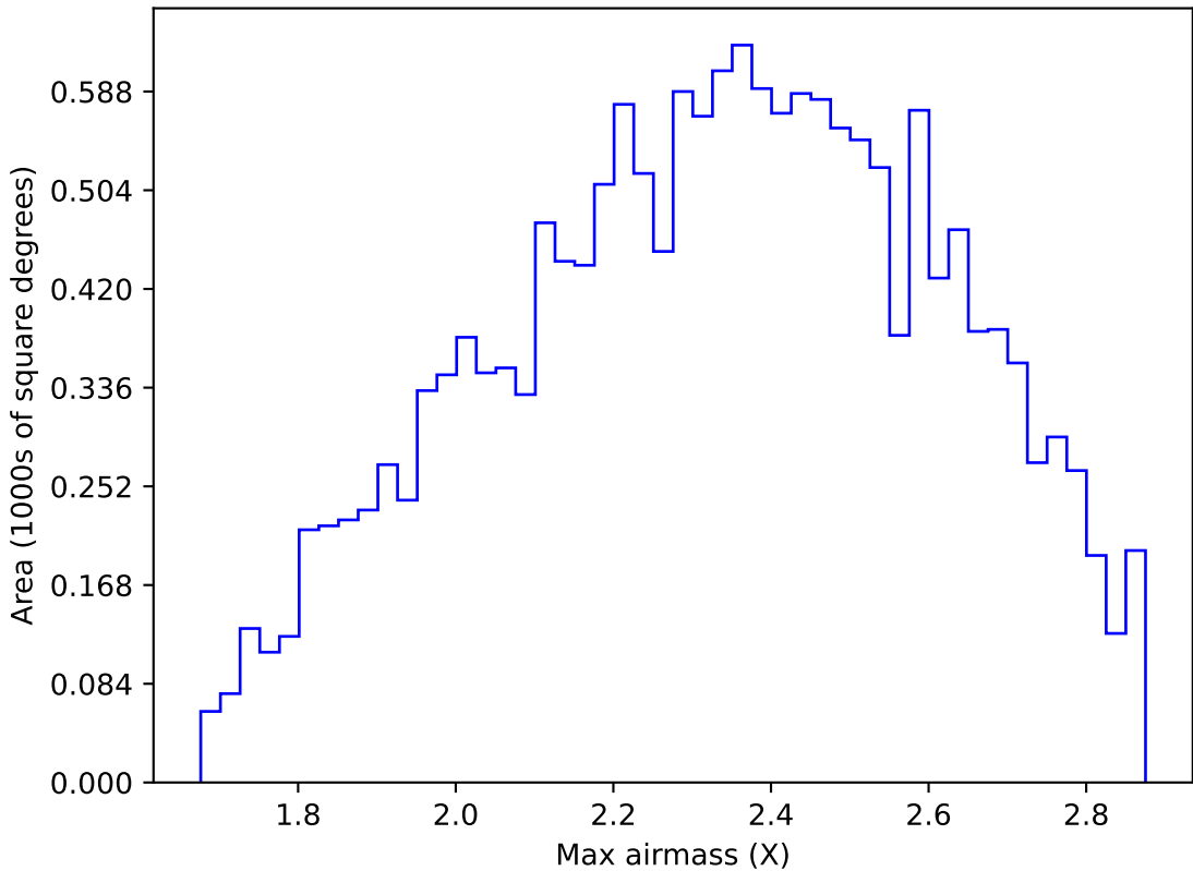
too_elab_r128_d3_ugrizy_v3.4_10yrs WFD y band: Max airmass
