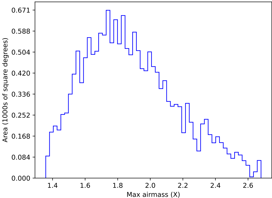
too_elab_r128_d3_ugrizy_v3.4_10yrs WFD u band: Max airmass
