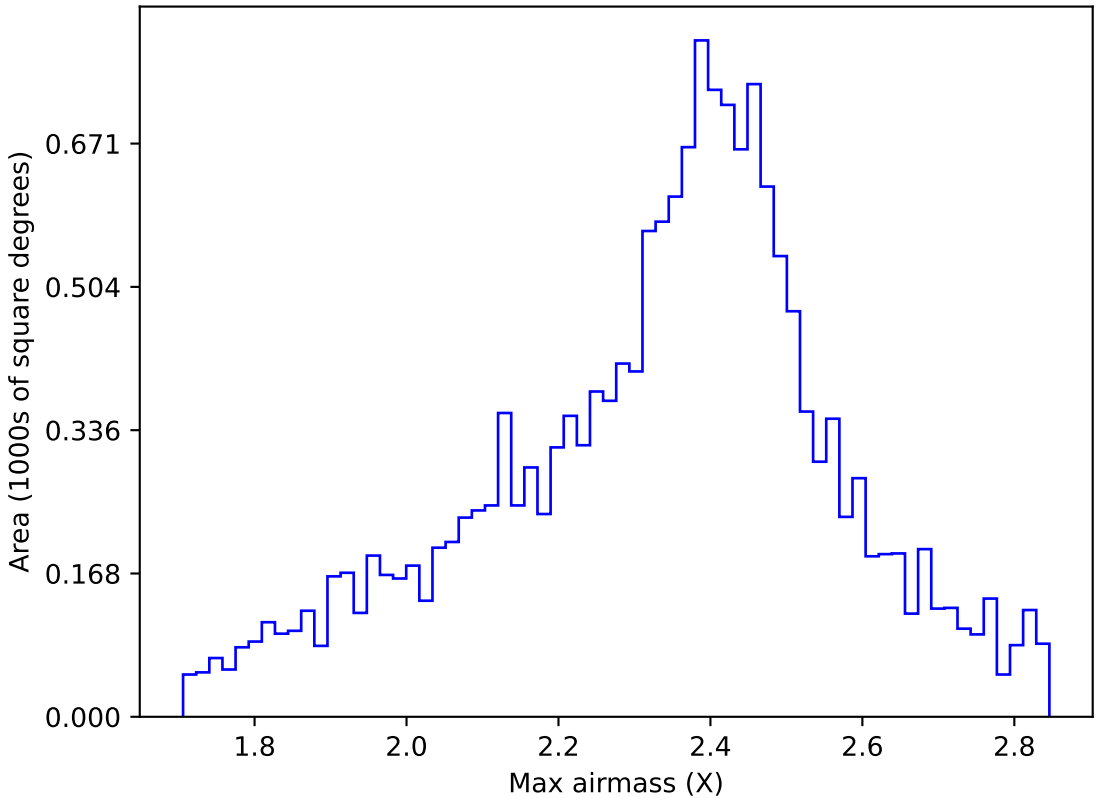
too_elab_r128_d3_ugrizy_v3.4_10yrs WFD r band: Max airmass
