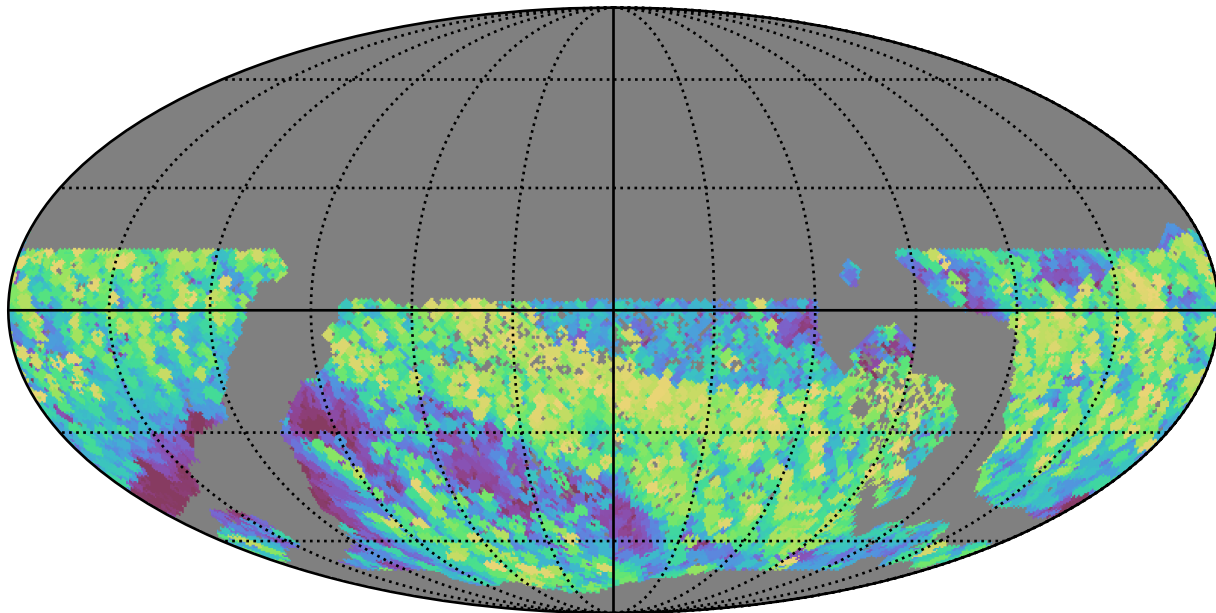
too_elab_r128_d3_ugrizy_v3.4_10yrs WFD i band: Max airmass
