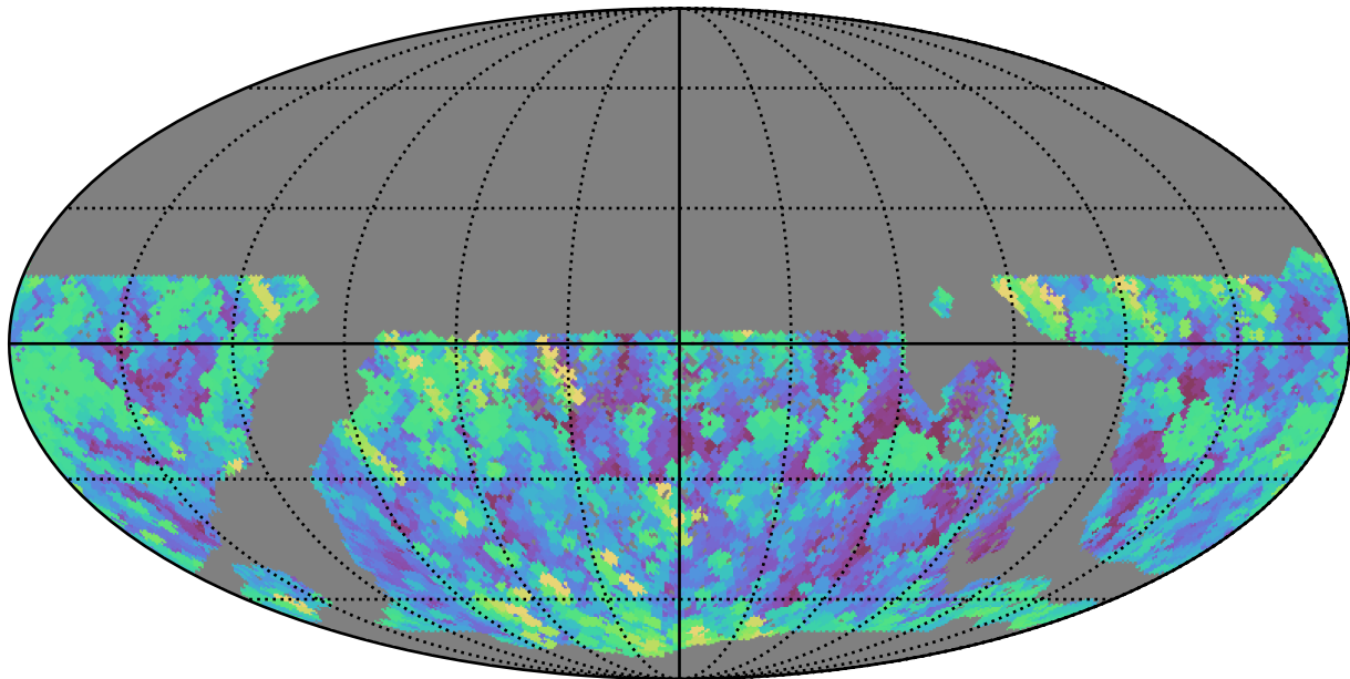
too_elab_r128_d3_ugrizy_v3.4_10yrs WFD g band: Max airmass
