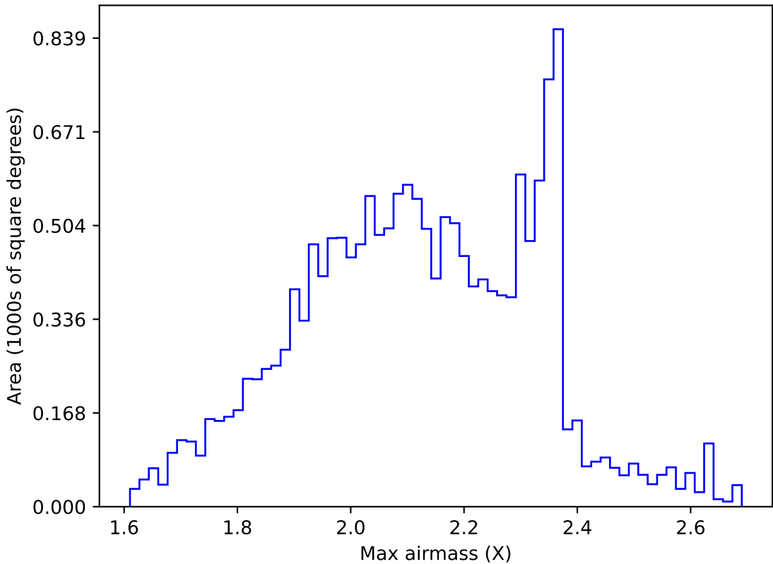
too_elab_r128_d3_ugrizy_v3.4_10yrs WFD g band: Max airmass
