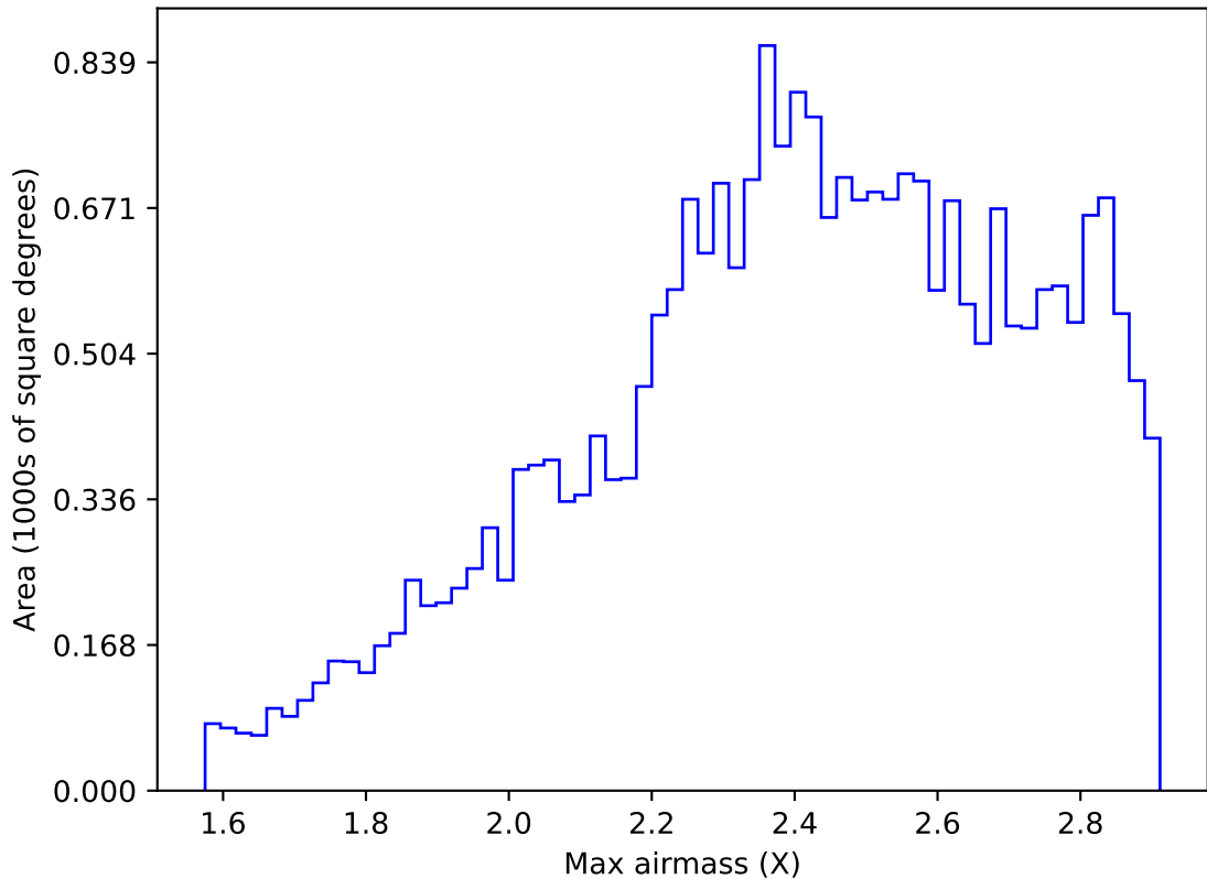
too_elab_r128_d3_ugrizy_v3.4_10yrs All sky z band: Max airmass
