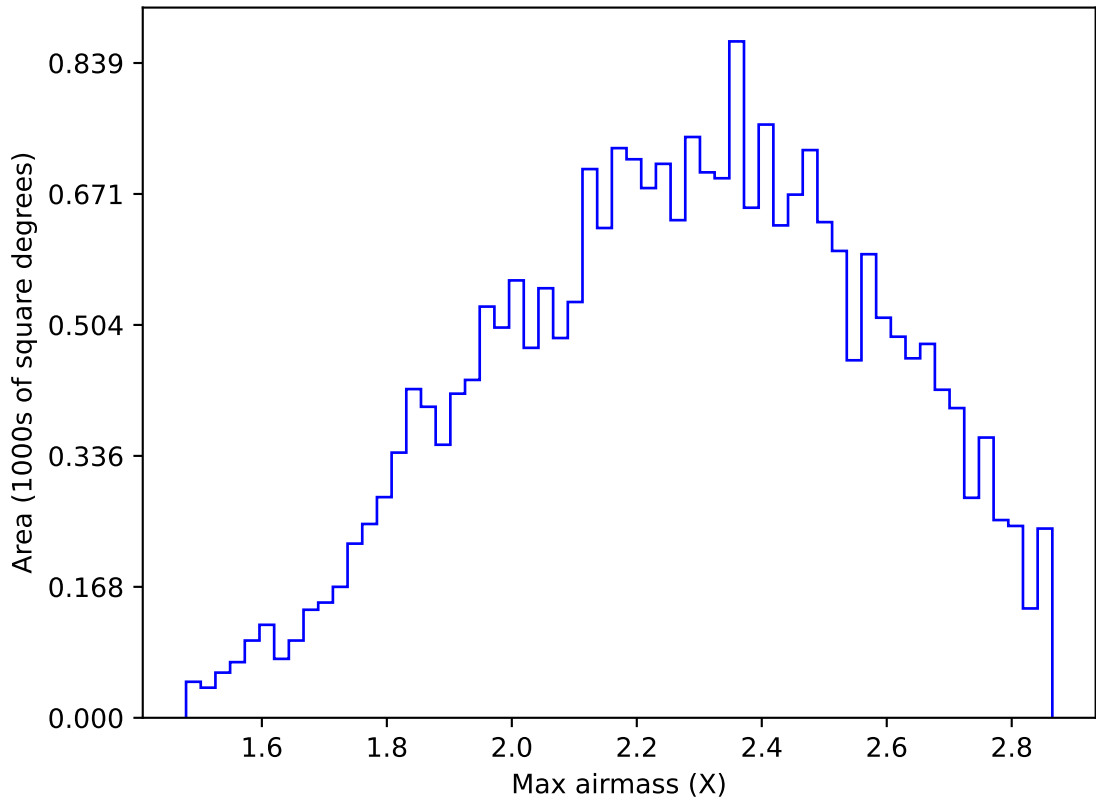
too_elab_r128_d3_ugrizy_v3.4_10yrs All sky y band: Max airmass
