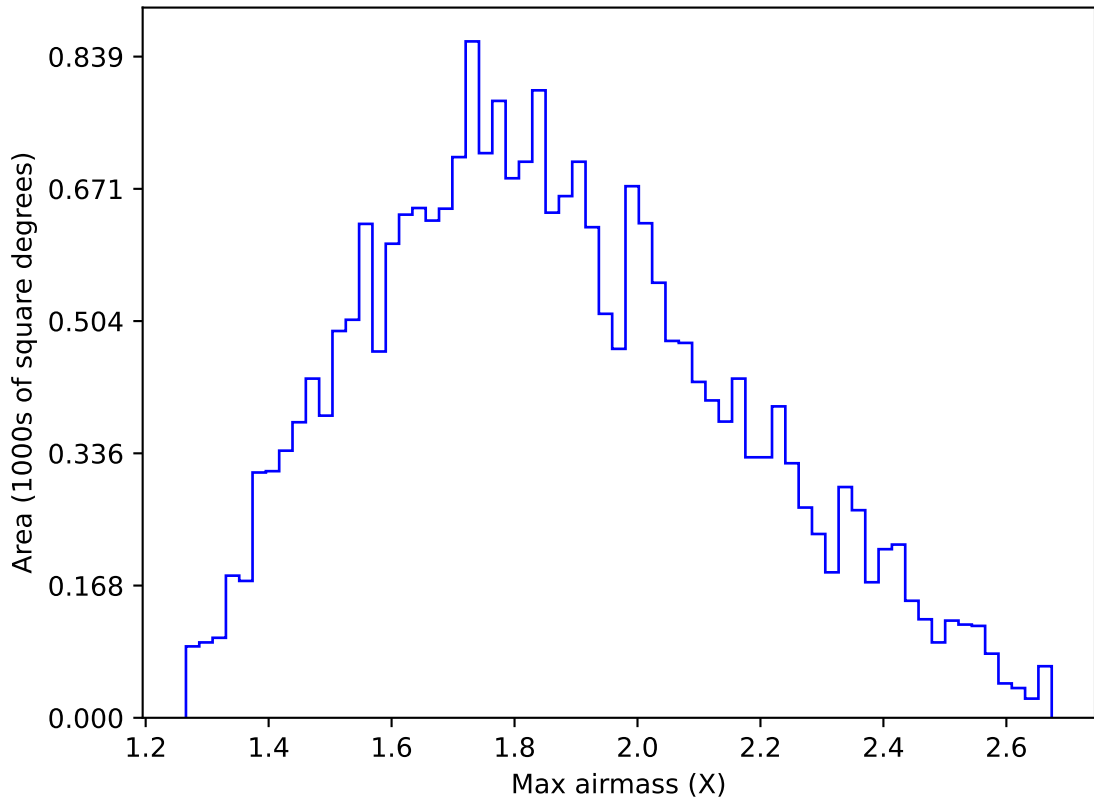
too_elab_r128_d3_ugrizy_v3.4_10yrs All sky u band: Max airmass
