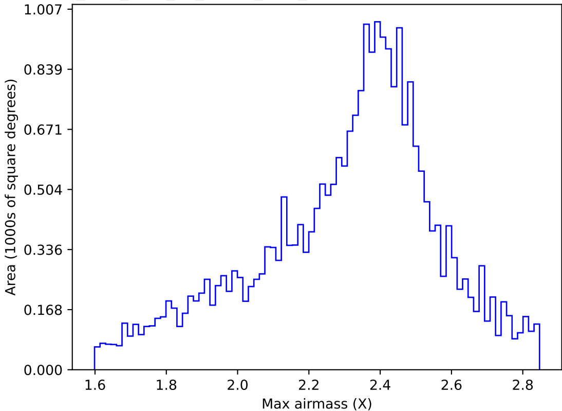
too_elab_r128_d3_ugrizy_v3.4_10yrs All sky r band: Max airmass
